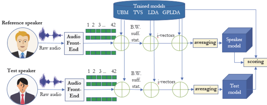
Figure 6 - Processing steps to compute the reference and the test speaker models, up to the scoring
